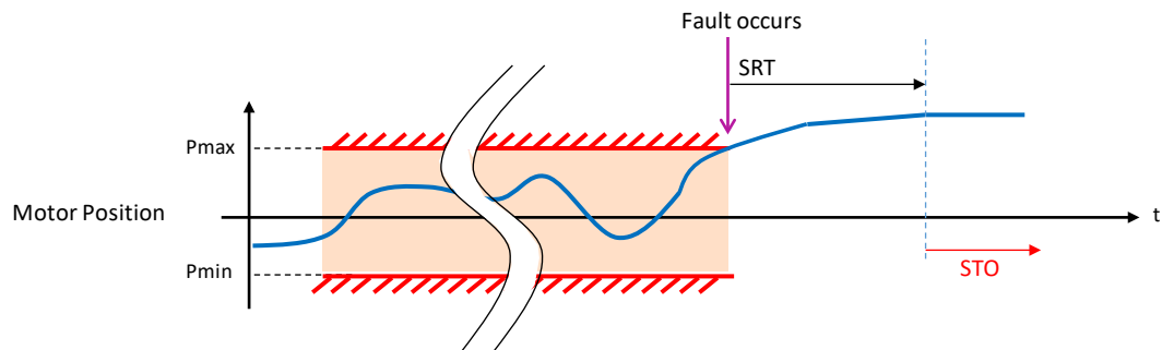
Fig. 1 Safety function response time of Safely-limited position
